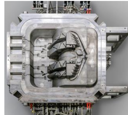
Torque box (E-car)
