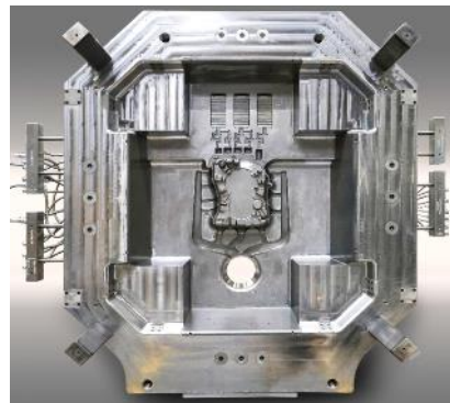
Volvo truck trans. housing (GF)
