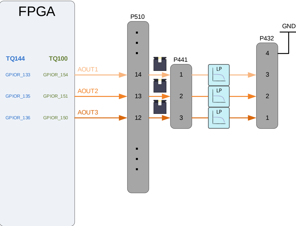
Figure 7: Analog out
