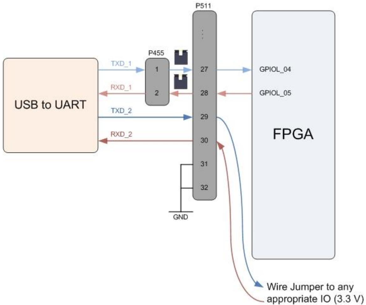
Figure 9: UART - T20Q100
