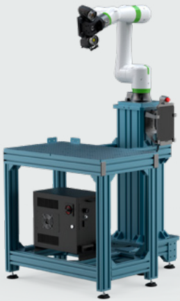
Automation Kit Comprehensive turnkey solution for automating the HandySCAN 3D and MetraSCAN 3D
