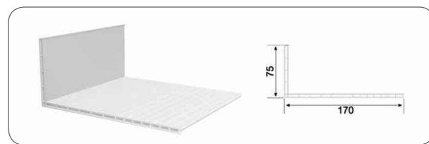
75 X 170 MM LINING PROFILE
