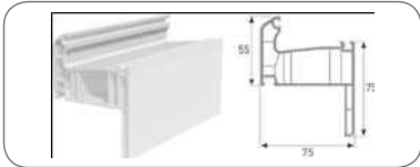
LINING FRAME PROFILE
