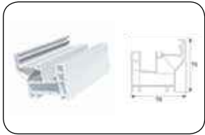
SLIDING FIX FRAME PROFILE
