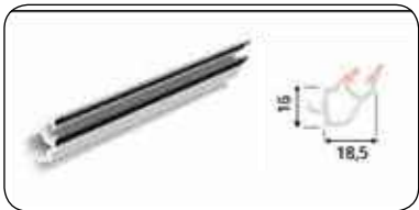
TRIPLE GLAZING BEAD PROFILE (32 MM)
