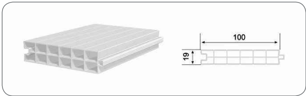
100X19 MM LAMBRI PROFILE
