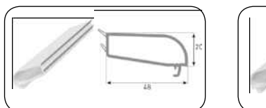
SINGLE GLAZING BEAD PROFILE (5 MM)
