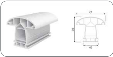
70 MULLION PROFILE
