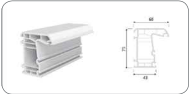
75 FRAME PROFILE
