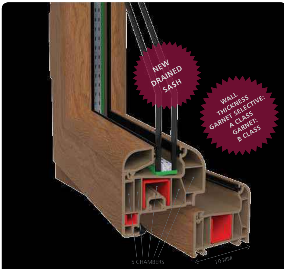
FRAME & SASH WIDTH 70 MM
