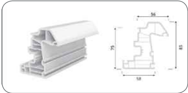
75 DRAINED SASH PROFILE
