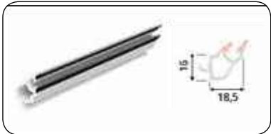
TRIPLE GLAZING BEAD PROFILE (32 MM)
