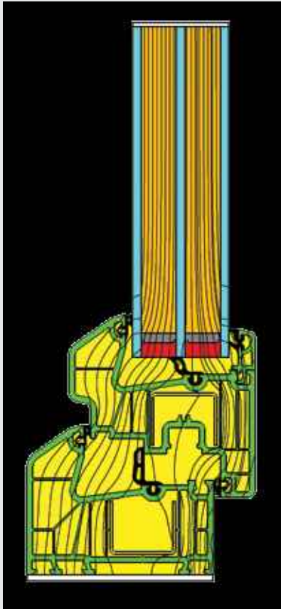
HEAT FLOW DIAGRAM
