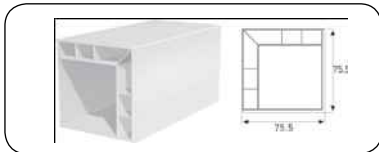
ANGLED POST BOX 90° PROFILE
