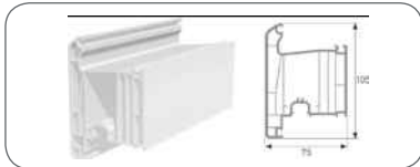
OUTSIDE OPENING DOOR PROFILE
