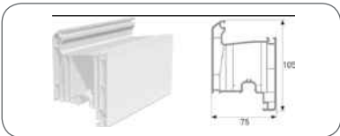
INSIDE OPENING DOOR PROFILE
