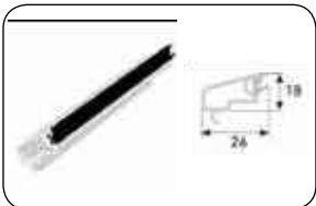
SINGLE GLAZING BEAD PROFILE
