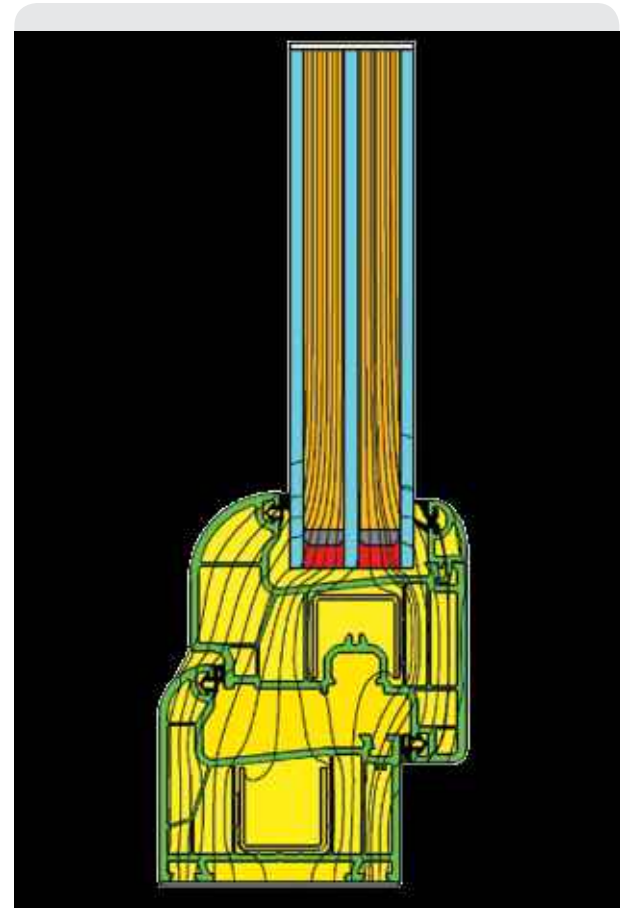
WINDOW HEAT FLOW DIAGRAM UF:1,2 W/M 2 °K UW: 1,05 W/M 2 °K
