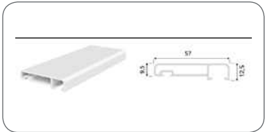
UPPER CLOSING PROFILE
