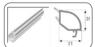
TRIPLE GLAZING BEAD PROFILE (32 MM)
