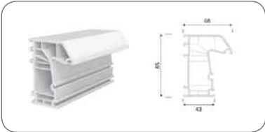
85 FRAME PROFILE
