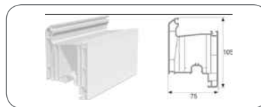
INSIDE OPENING DOOR PROFILE
