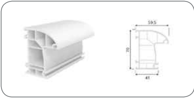
70 FRAME PROFILE
