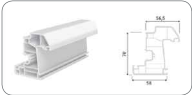
DRAINED SASH PROFILE
