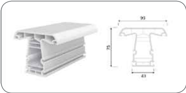
75 MULLION PROFILE
