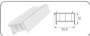
FRAME BASE MONTAGE PROFILE
