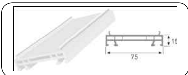
FRAME ELEVATION PROFILE (15 MM)
