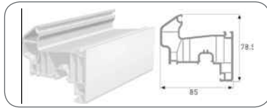
DRAINED SASH PROFILE
