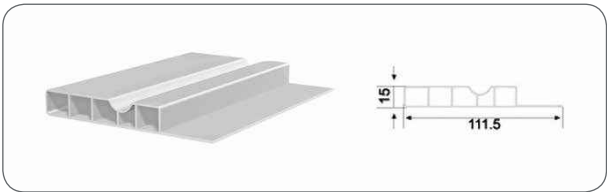
INDOOR SILL PROFILE
