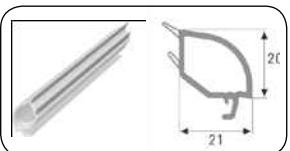
TRIPLE GLAZING BEAD PROFILE (32 MM)
