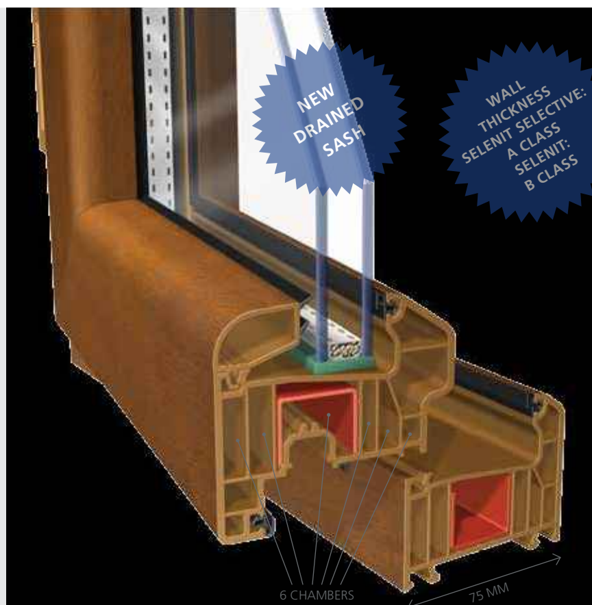
FRAME & SASH WIDTH 75 MM
