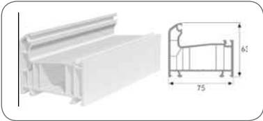
FRAME PROFILE
