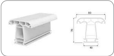
MULLION PROFILE
