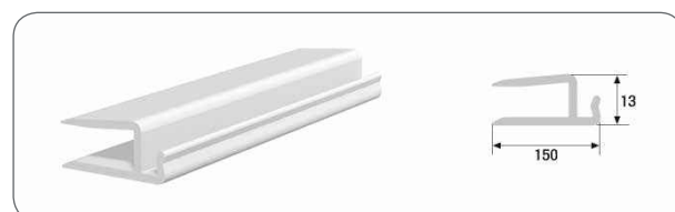
LINING ADAPTING PROFILE
