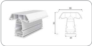
85 MULLION PROFILE
