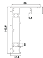
GIO-PLUS SIDE MAST PROFILE 608
