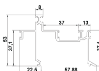
GIO-PLUS SIDE MAST ADAPTER PROFILE 611-1
