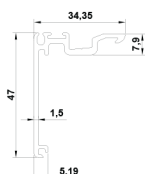
GIO-PLUS CLAMP PROFILE 609
