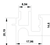
GIO-PLUS HINGE PROFILE - 1 614-1
