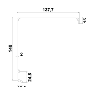
GIO-PLUS MOTOR ENCLOSURE PROFILE 615-1
