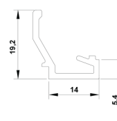
GIO-PLUS GLASS ADAPTER PROFILE 616
