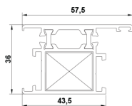
GIO-PLUS LEAF PROFILE 606
