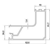
GIO-PLUS FIRST CHANNEL PROFILE 610
