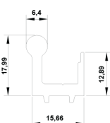
GIO-PLUS HINGE PROFILE - 2 614-2
