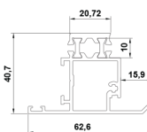
GIO-PLUS FIRST LEAF ADAPTER PROFILE 607
