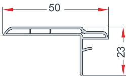
CASING PROFILE WITH CLIP KLİPSLİ PERVAZ PROFİLİ EN 52
