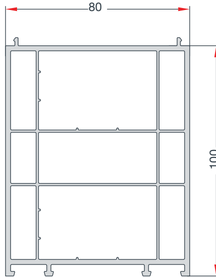
80 x 100 FRAME EXTENSION PROFILE 80 x 100 GENİŞLETME PROFİLİ EN 115 HIGHLINE
