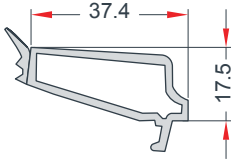
4-mm DECORATIVE SINGLE GLAZING BEAD 4 mm DEKORATİF TEK CAM ÇİTASI EN 39
