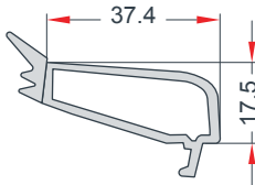
4-mm UNIVERSAL SINGLE GLAZING BEAD 4 mm ÜNİVERSAL TEK CAM ÇİTASI EN 42
