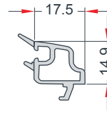
24-mm DECORATIVE DOUBLE GLAZING BEAD 24 mm DEKORATİF ÇİFT CAM ÇİTASI EN 43
