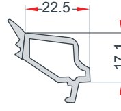
20-mm DECORATIVE DOUBLE GLAZING BEAD 20 mm DEKORATİF ÇİFT CAM ÇİTASI EN 40
