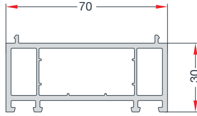
30 x 70 FRAME EXTENSION PROFILE 30 x 70 GENİŞLETME PROFİLİ EN 111 KLASLINE
