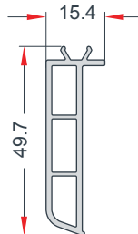
CASING PROFILE WITH CLIP KLİPSLİ PERVAZ PROFİLİ EN 30
