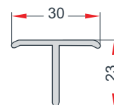
"T" CLOSING PROFILE DAR "T" KAPAMA EN 63
