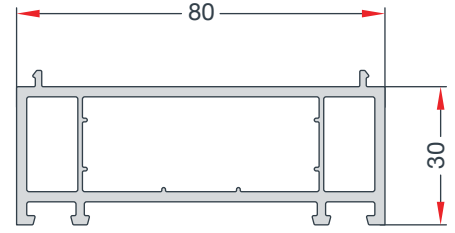
30 x 80 FRAME EXTENSION PROFILE 30 x 80 GENİŞLETME PROFİLİ EN 112 HIGHLINE
