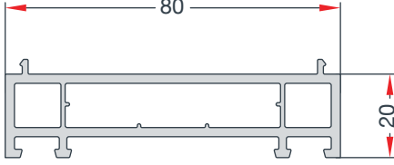
20 x 80 FRAME EXTENSION PROFILE 20 x 80 GENİŞLETME PROFİLİ EN 110 HIGHLINE
