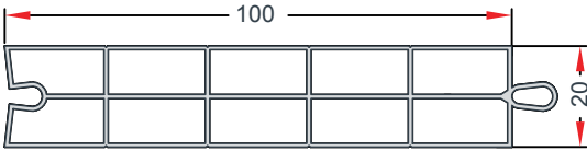
10-cm PANEL PROFILE 10 cm LAMBRI PROFİLİ EN 60
