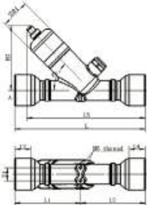
VPF400 with sight glass
