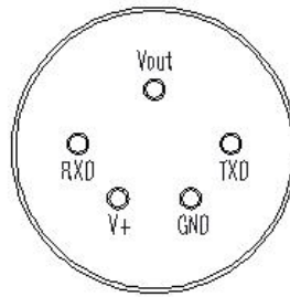
Bottom view from pin surface
