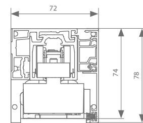
Wandmontage 54 mm
