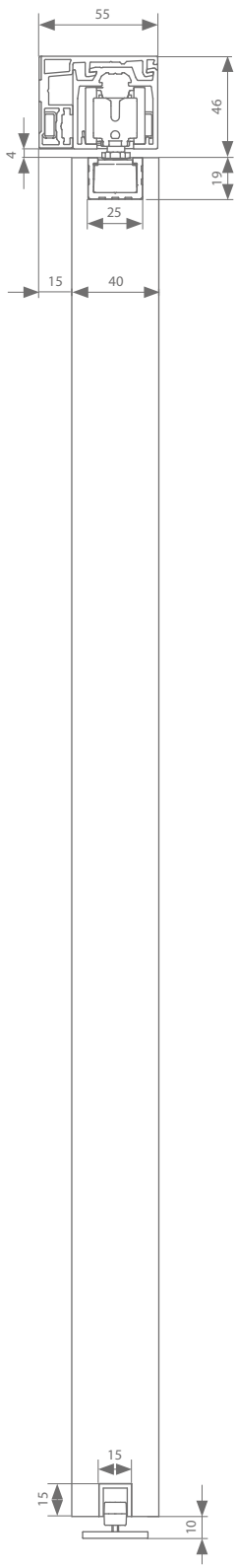
Wandmontage 40 mm
