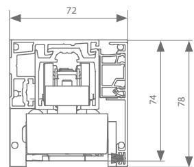
Wandmontage 50 mm
