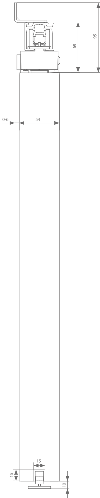
Wandmontage 54 mm
