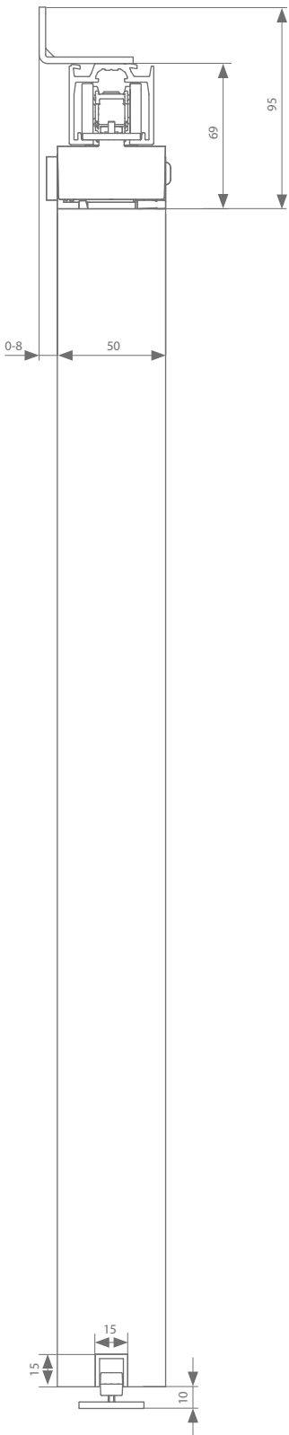
Wandmontage 50 mm
