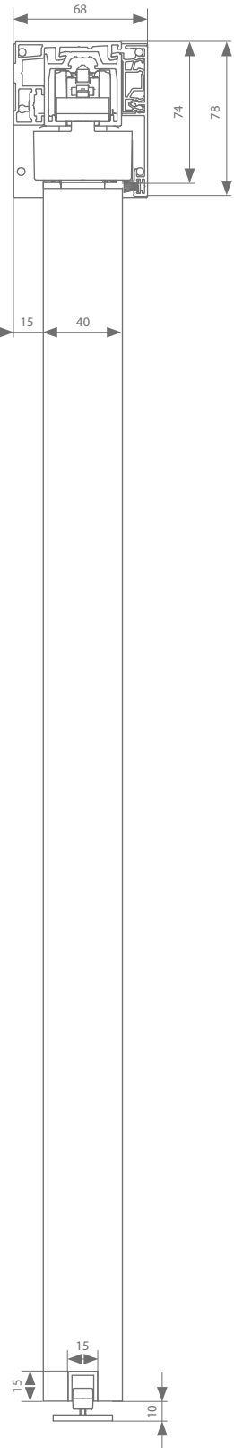
Wandmontage 40 mm
