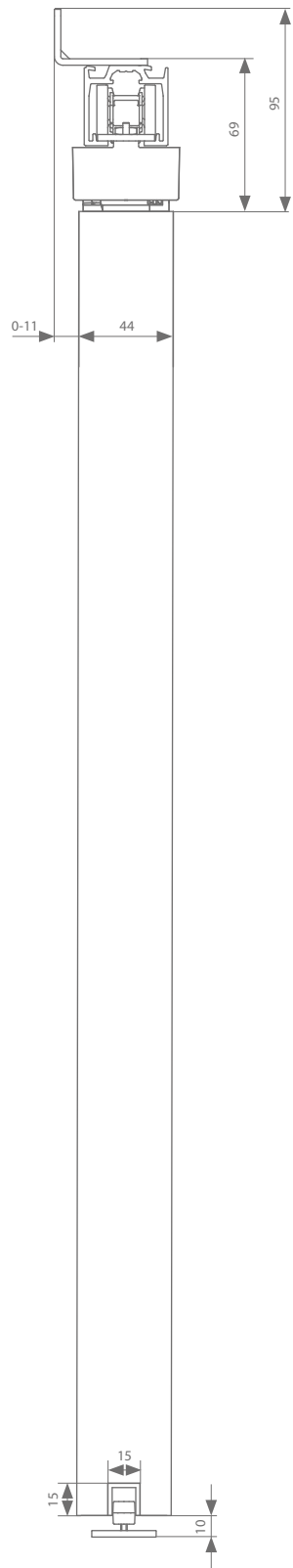
Wandmontage 44 mm
