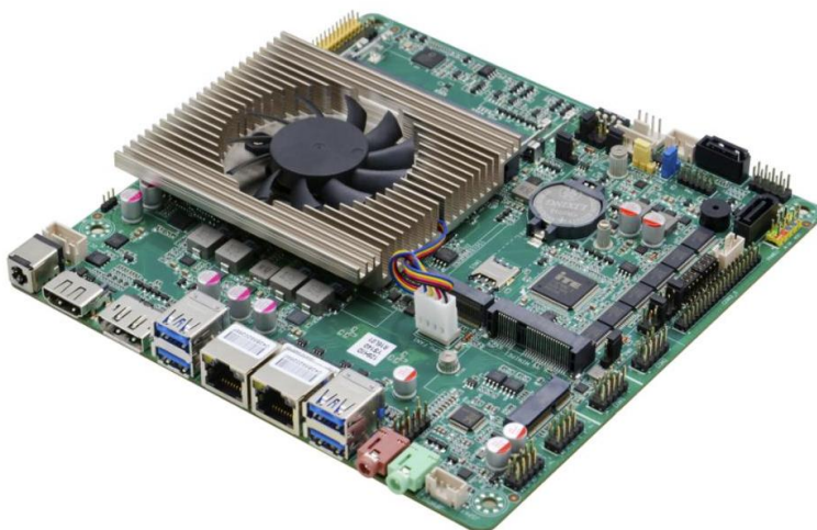
ITX-YS140R1_I526L VER:1.0 I/O View
