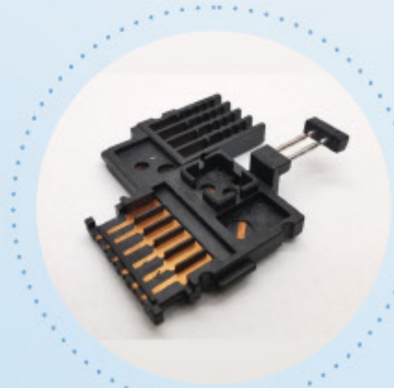
connector overmolding
