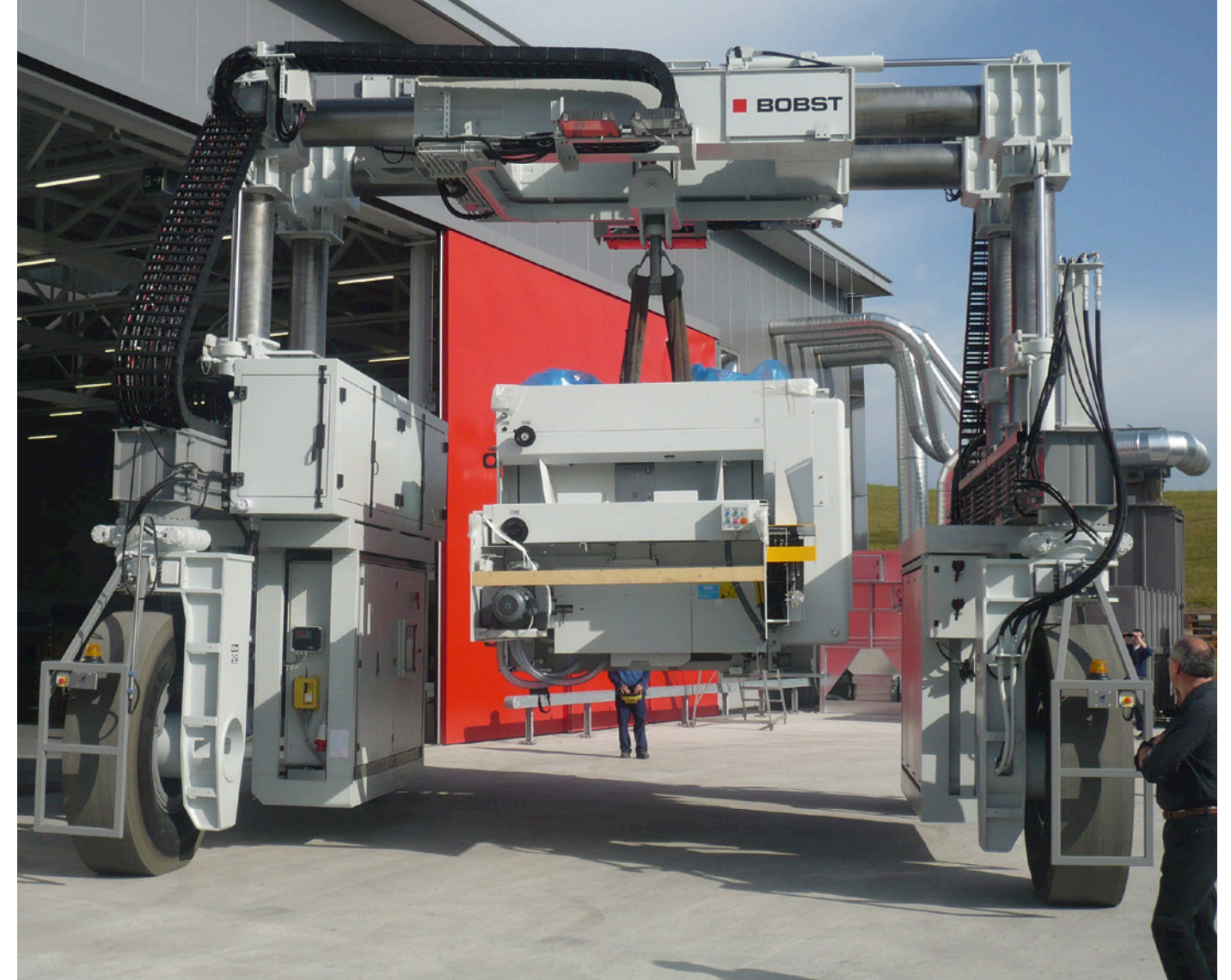
MOBILE STRADDLE TRANSPORTER Capacity: 60 t - SWITZERLAND Mobile straddle transporter with hydraulically adjustable height and width
