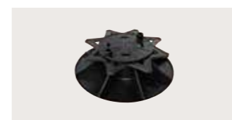
Height-adjustable deck support P 9431 55 to 95 mm pivoting base
