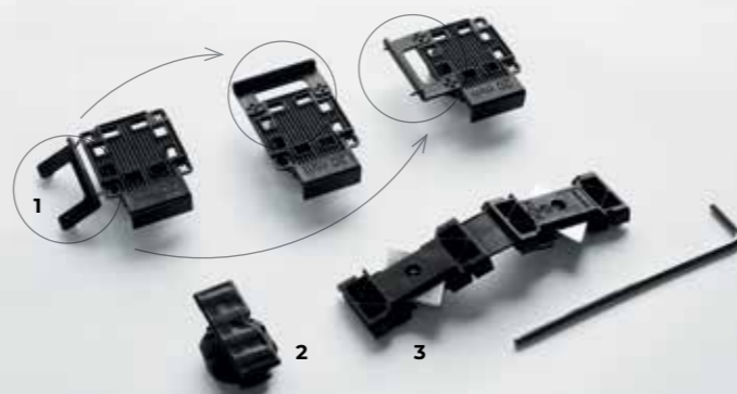
1: multi-adjustable vertical clip, 2: horizontal rotating clip, 3: flexible corner clip connection plate
