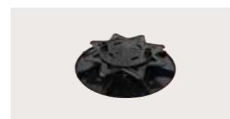
Height-adjustable deck support P 9430 35 to 55 mm pivoting base
