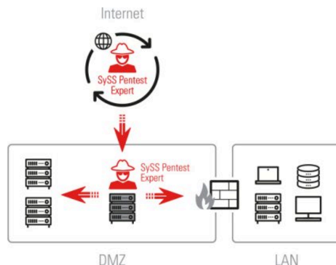
Figure 2.44: Module PIVOT
