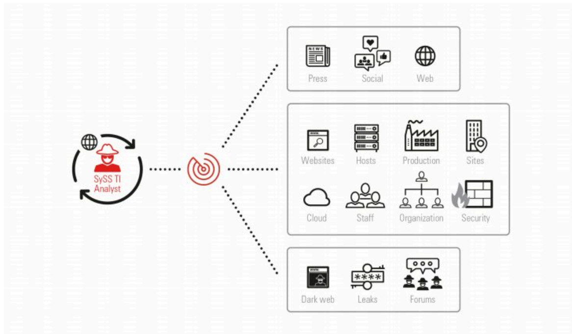
Figure 4.1: Module TI/RECON
