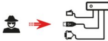
Figure 2.31: Module ES/EXTERNAL
