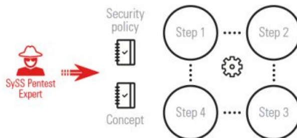
Figure 2.45: Module REVIEW
