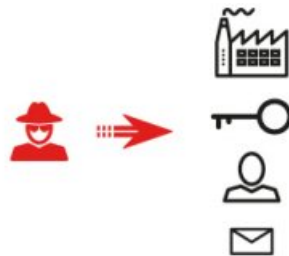
Figure 2.42: Module SOCIAL
