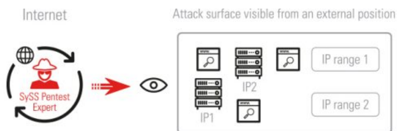
Figure 2.41: Module RECON
