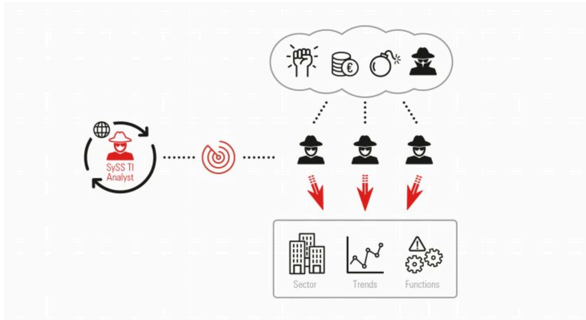
Figure 4.2: Module TI/LANDSCAPE
