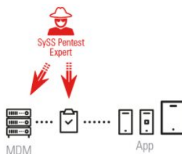
Figure 2.23: Module MOBILE/MDM
