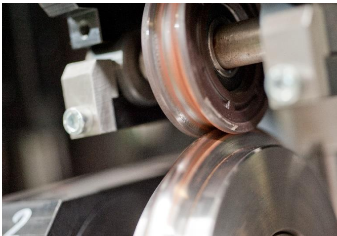
Endurance test
