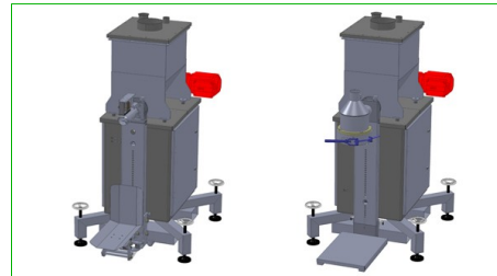
Kombischneckenpacker Combined screw packers
