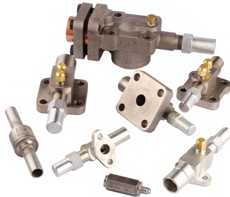
压缩机吸排气阀 Compressor suction and discharge valve 制冷剂 Refrigerants : CFC, HCFC, HFC, R744 温度范围 Working temperature range : -40℃ ~ +140℃ 规格尺寸 Specification and size : DN6 ~ DN80 压力范围 Pressure range : 0 ~ 16.0 MPa 优点 Features and advantages : 耐低温球铁和锻造低温钢材质 low temperature resistant ductile iron and low temperature forged steel 双密封耐用寿命长 dual sealing and long service life CE CERTIFICATION
