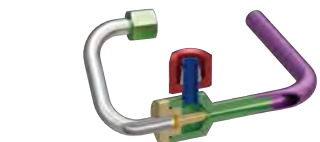
功能接头 Functional connector 制冷剂 Refrigerants: CFC, HCFC, HFC 温度范围 Working temperature range: -29°C ~ +120°C 规格尺寸 Specification and size: DN1 ~ DN25 压力范围 Pressure range: 0 ~ 4.5 MPa ( 液压hydraulic pressure 6.3 ) 优特点 Features and advantages: 特氟龙预涂密封良好 Pre-glued PTFE has a good sealing performance 无氧钎焊坚固耐用 Oxygen-free brazing will make products sturdy and durable 精度高 high precision 可靠性强 strong reliability CE certification
