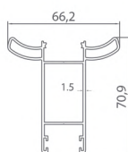
SUISS MAST PROFILE WITH DOUBLE HANDLE
