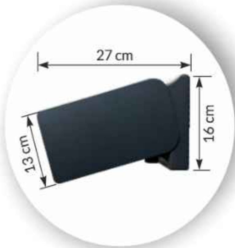
Wandmontage
