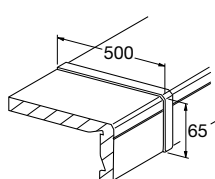
Window sill connection profiles
