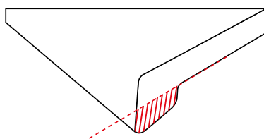
Milling the front edge flush ****
