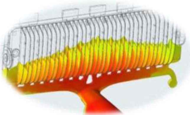
Aluminium 44 300 /3,250kg
