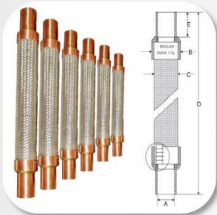
VIBRATION ABSORBER
