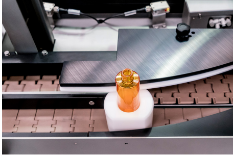
Puck introduction system
