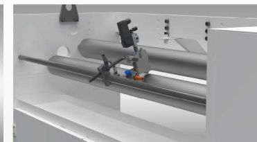
Otomatik Yan Tutkal Nozzle Sistemi (Std.) Automatic Side Glue System with Nozzle
