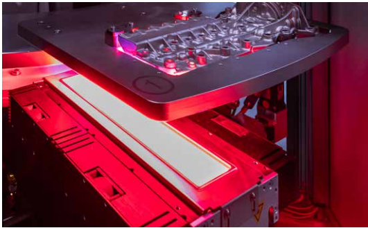
Plane surface inspection using an F sensor
