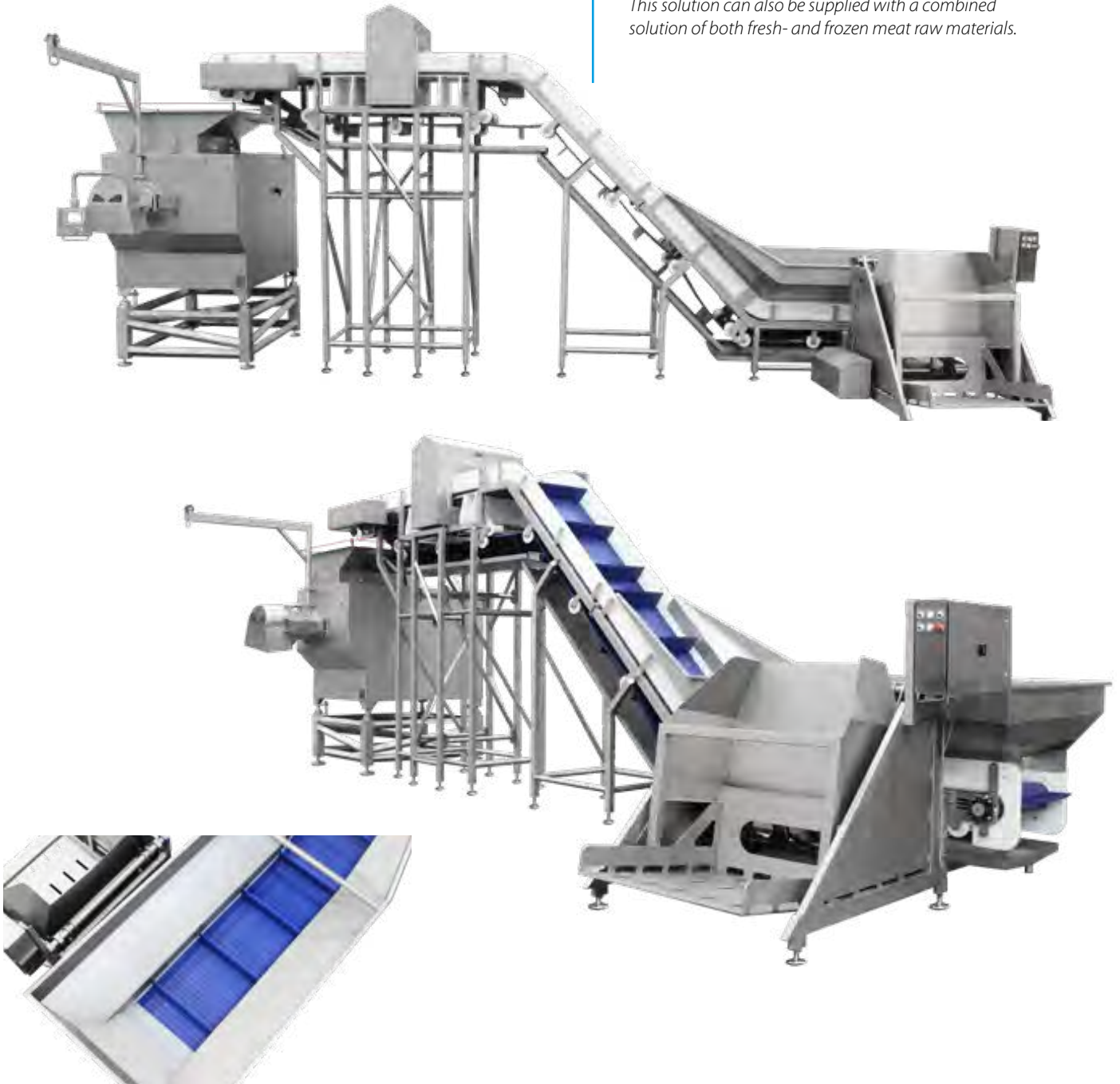
Top view of scanSwing loader and belt conveyor
