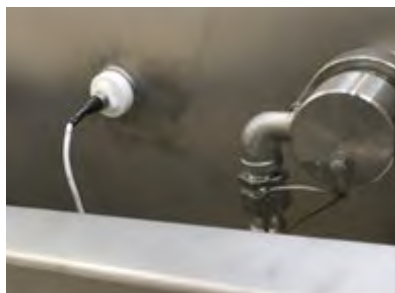
Valve shown mounted on mixer. Temperature sensor shown to the left and valve shown to the right.
