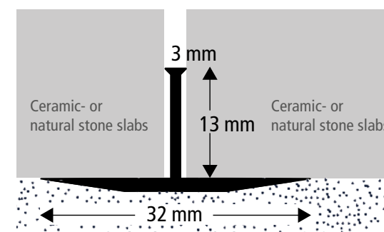
joint profile
