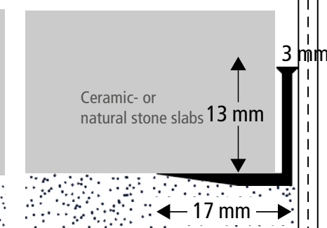
L-profile for façade connection
