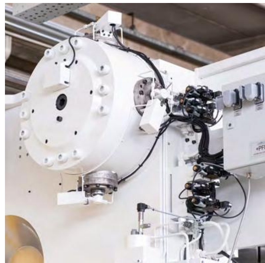
Sfilamento colonna superiore. Removal of upper tie bar.
