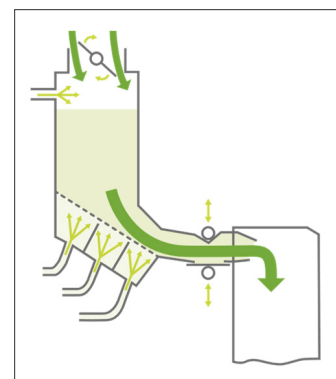
Functionality of pneumatic BVP/V conveying
