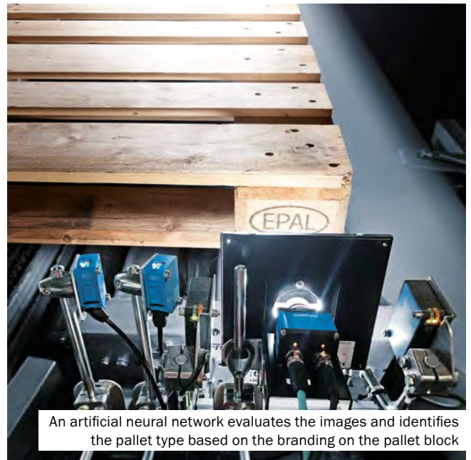
PACS can be mounted at any position along the conveyor system and captures images of the pallet blocks from two sides
