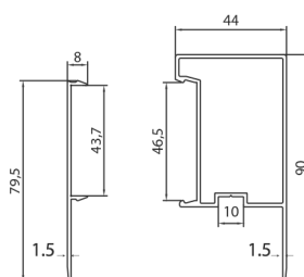
CASE ADJUSTMENT PROFILE 104
