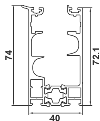
AURA-PLUS CASE PROFILE 201
