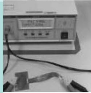
Peel Force Tester 剝離力測試儀
