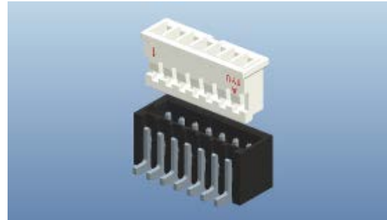
KM2003 series (2.0mm)
