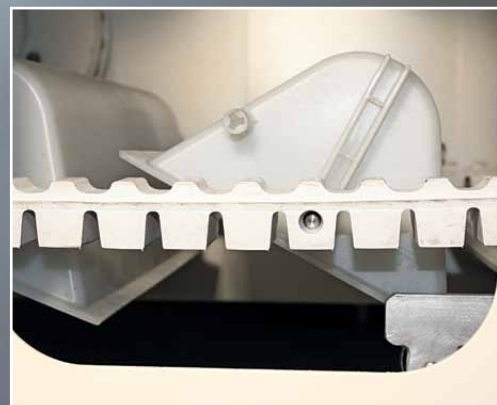
Buckets are emptied by the tilting mechanism
