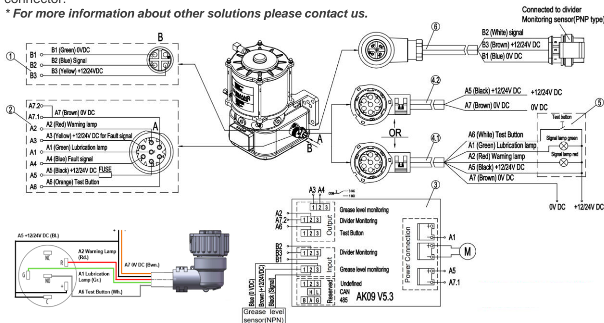
Dia. 26.1 Wiring Diagram for ALPB BYN controller version
