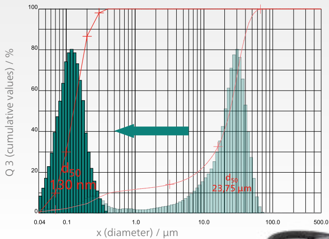
Particles size measuring method CILAS 1064 wet Measuring range: 0.04 μm – 500.00 μm
