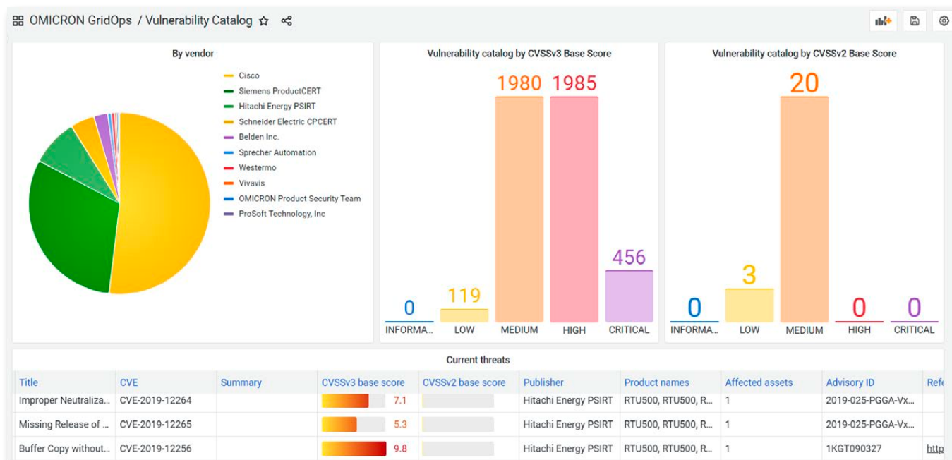
GridOps Schwachstellen-Dashboard
