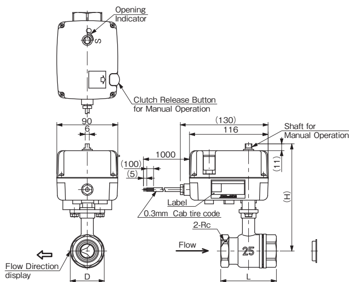
Two-way Valve
