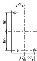
Panel Cut Dimension
