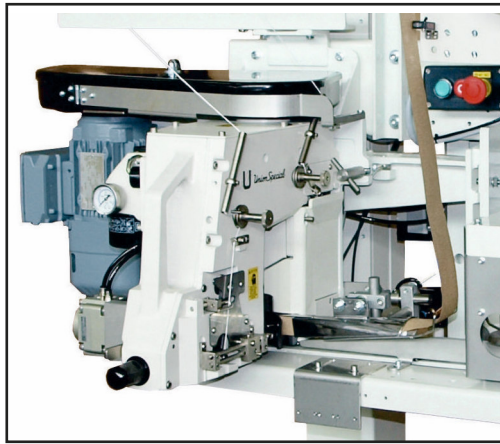
BC211UA23-1NW High performance automatic, single needle, two thread bag closing machine for closing bags with crepe paper tape
