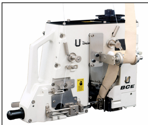
BCE311KA12-1M Improved „Economy“ automatic bag closing machine for seaming and placing a self-adhesive crepe tape over the sewn closure.
