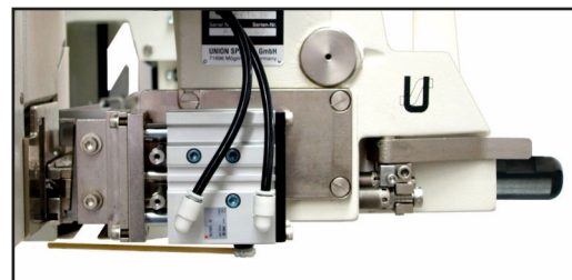
Electro-pneumatically operated guillotine. For machine styles: BC211U/UA25, BC211U/UA26, BC211PD26 BCE311UA25, BCE311U/UA26
