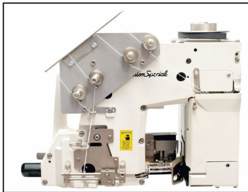
BC211PD26-2M High performance automatic, two needle, four thread bag closing machine for closing filled bags.
