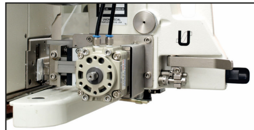
Electro-pneumatically operated fast guillotine. For machine styles: BC211U/UA23, BC211U/UA24 BCE311UA23, BCE311UA24
