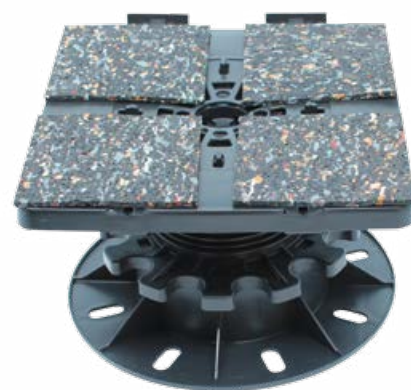
Figure right: Porto-support PLUS with top plate and granulate pads (supplied with the top plate)
