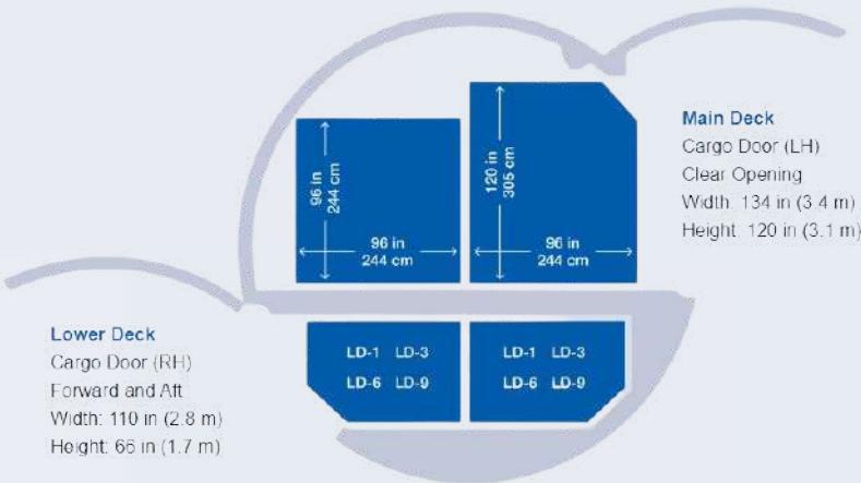
Cross Section Showing Main Deck and Lower Compartment
