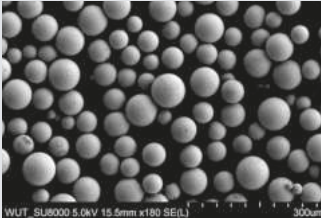
Maximum spherical Ideal for LPBF, BJ, MIM, and other Additive Manufacturing processes
