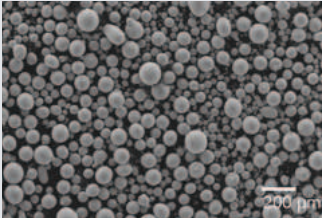
Highly spherical deal for LPBF, BJ, MIM, and other Additive Manufacturing processes
