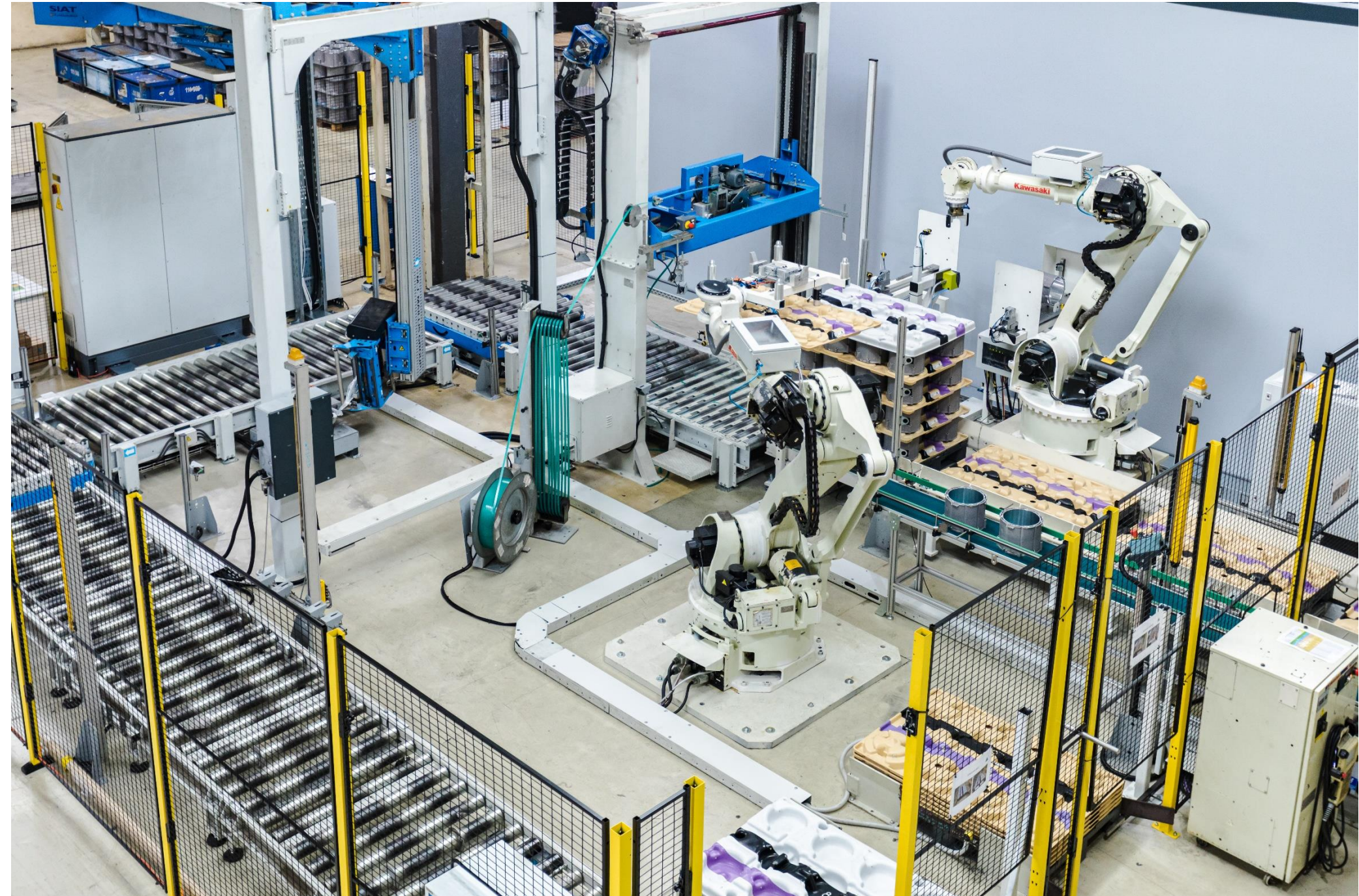
Automated packaging station – VW MEB
