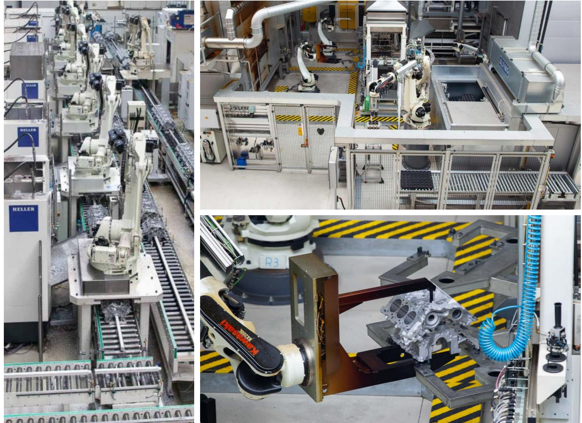
Engine Block V6/V8 - Audi/Porsche
