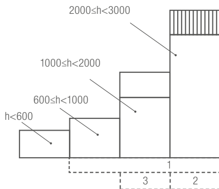
b) Fall protection for equipment that is difficult to access
