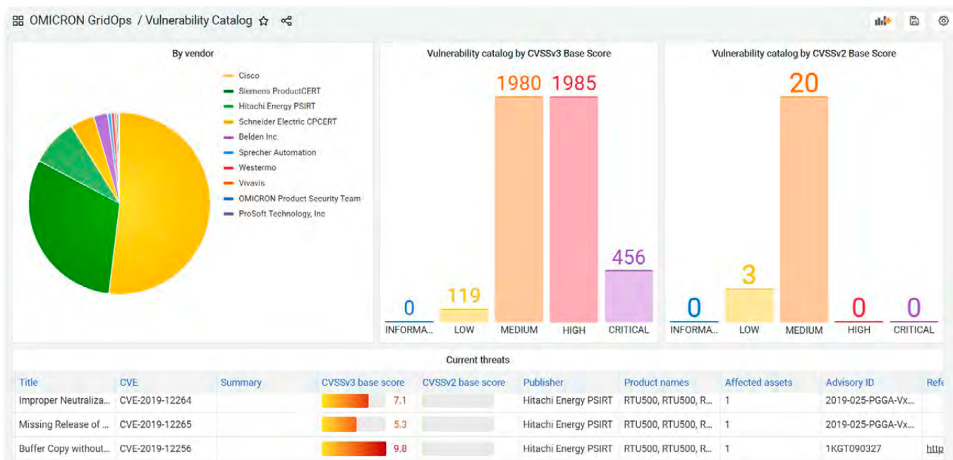
GridOps Schwachstellen-Dashboard
