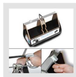
Planet installation box with precisely accurate length tool and built-in saw guide (Page 13)
