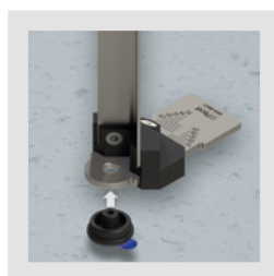
Positioning tool for adhesive base (Page 12)
