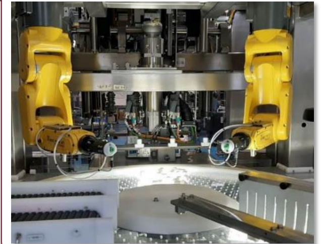
Feed Flex robotic cap orienter with vision system
