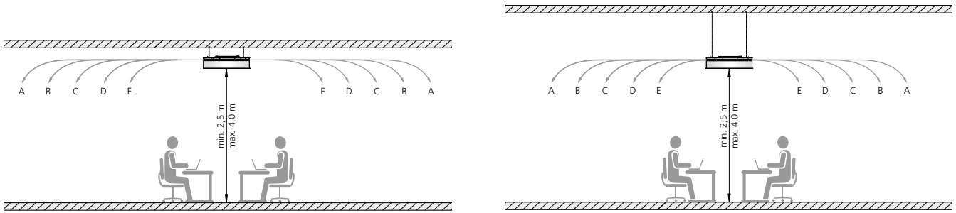
Example of suspension height and throw distances
