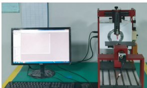
水滴角测试仪 Water drop angle tester
