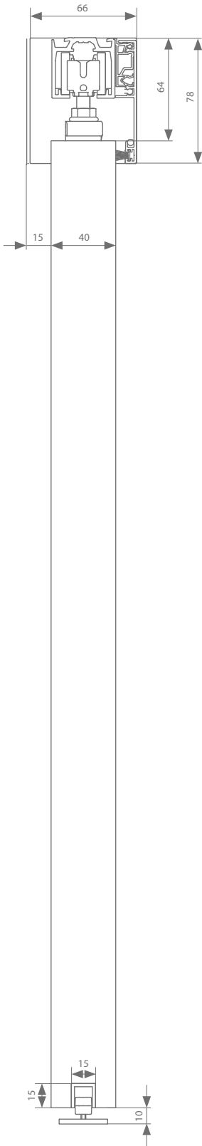
Ceiling mount 40 mm
