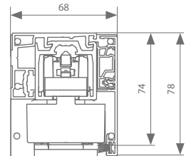
Wall mount 40 mm
