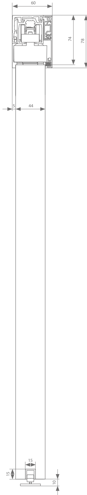
Wall mount 44 mm
