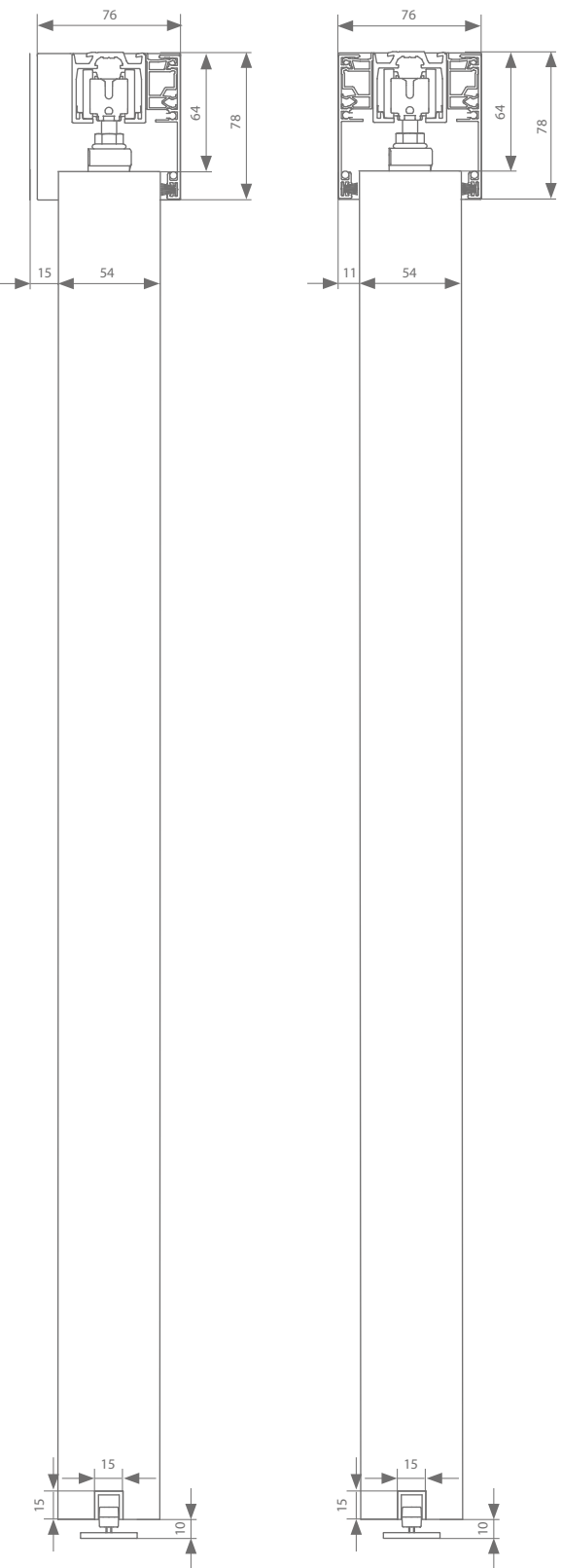
Ceiling mount 54 mm
