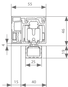
Wall mount 40 mm
