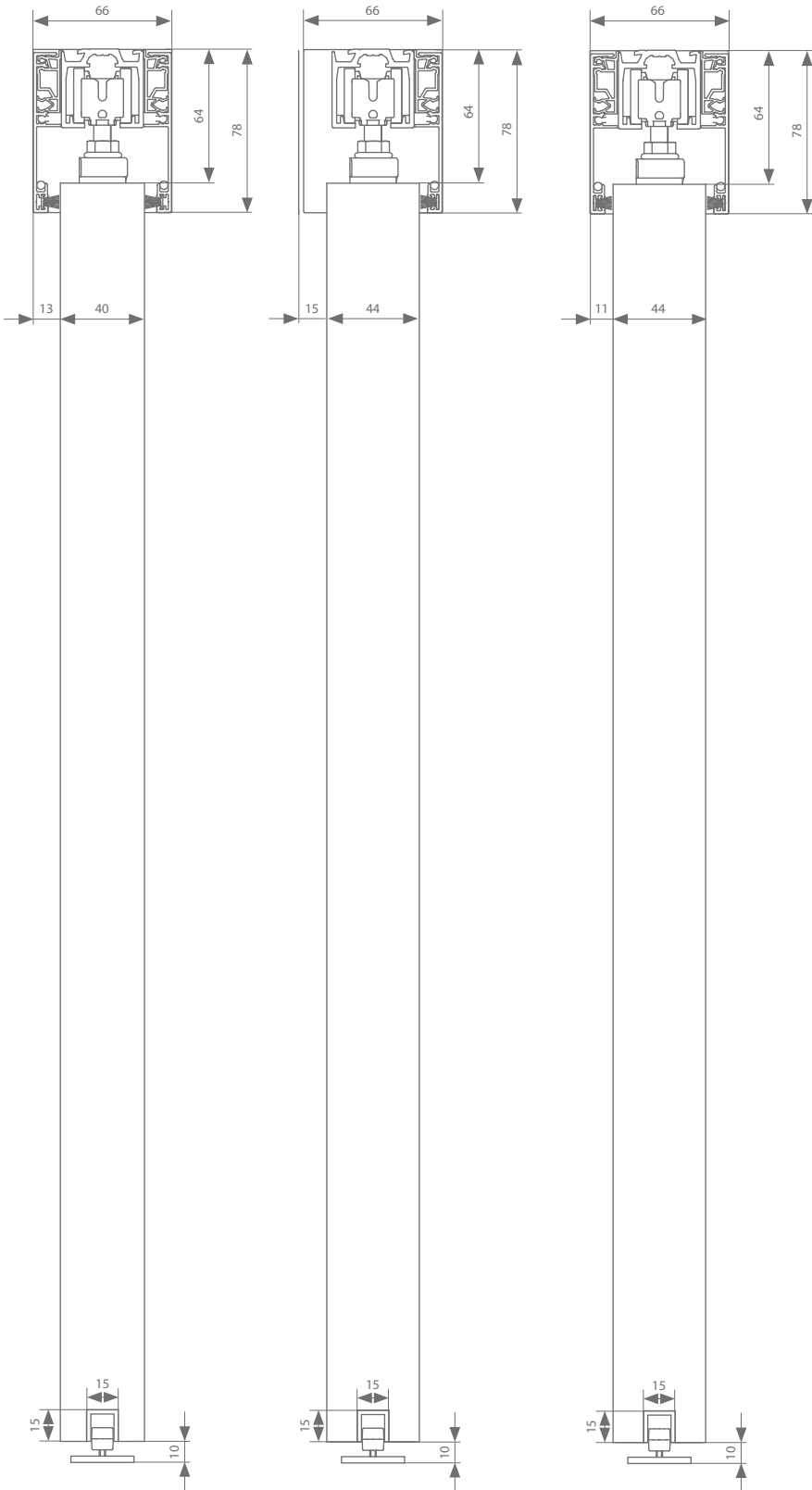
Ceiling mount 44 mm
