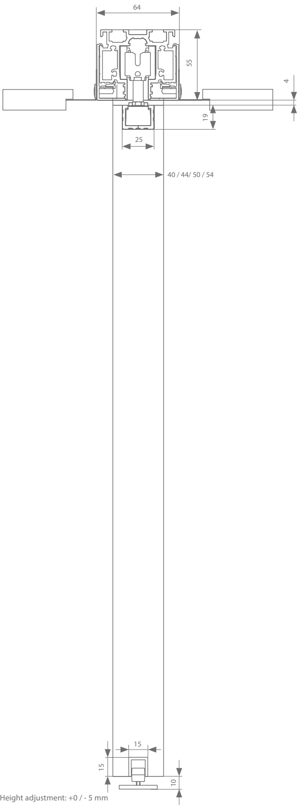
For suspended ceiling (1+2)
