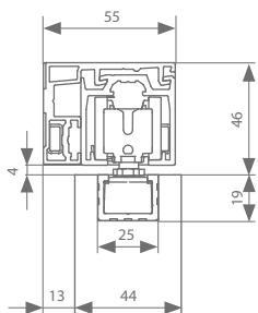
Wall mount 44 mm
