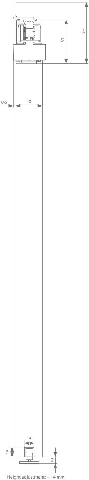
Wall mount 40 mm
