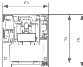
Wall mount 44 mm
