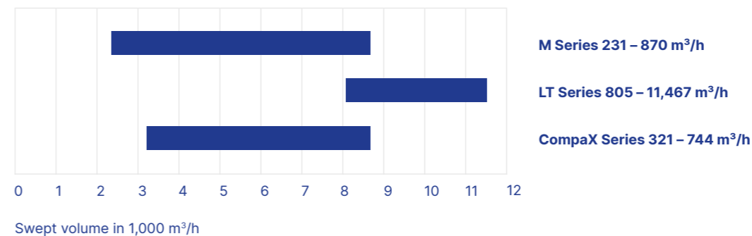
Swept volume ranges
